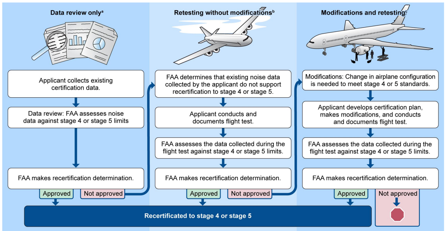
Figure 1: Overview of FAA’s Process for Recertificating Airplanes to Stage 4 or Stage 5 Noise Standards
