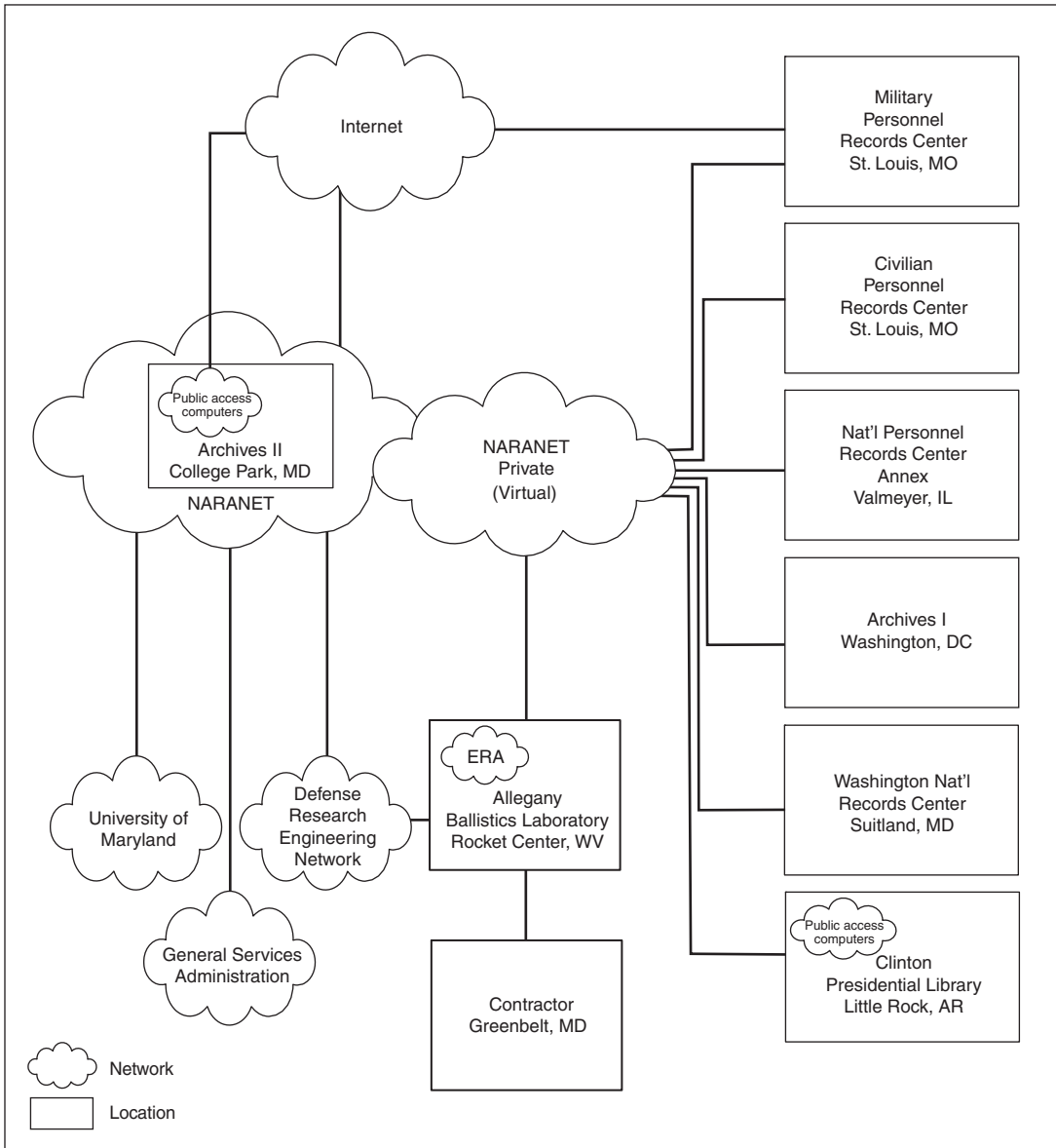
Figure 1: Simplified NARA Network Diagram
