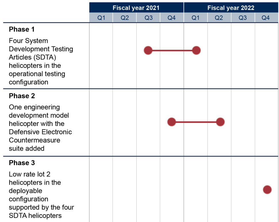
Figure 2: Schedule and Configuration of the Three Phases of Operational Testing for the CH-53K
