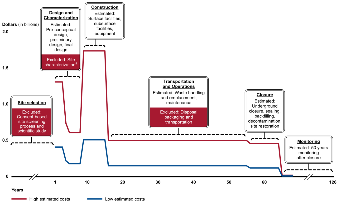
Figure 5: Department of Energy's (DOE) High- and Low-Range Cost Estimates for Developing a Defense High-Level Waste Repository, Along with Activities for which DOE Did Not Estimate Costs (in billions, 2013 dollars)
