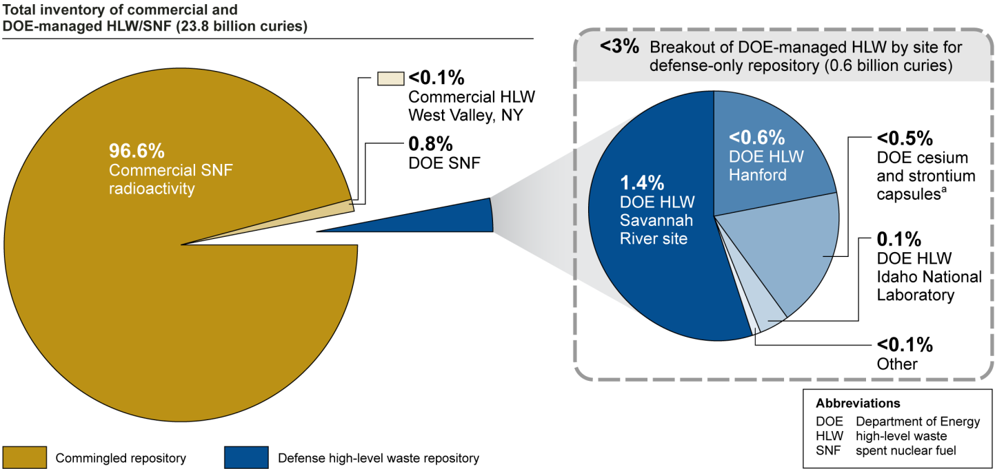
Figure 3: Radioactivity of High-Level Waste (HLW) and Spent Nuclear Fuel (SNF) Planned for Separate Defense and Subsequent, Mostly Commercial Repositories (by Curie and Type of Repository)
