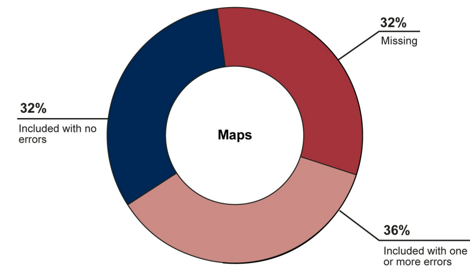
Figure 5: Estimated Errors in Maps from the National Oceanic and Atmospheric Administration (NOAA) Weather Modification Database
