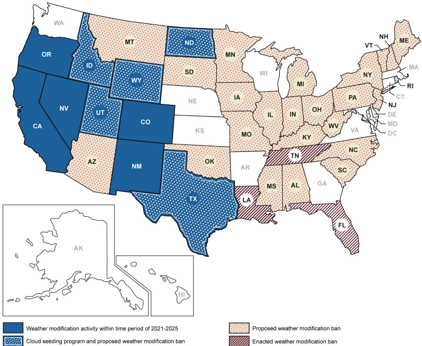
Figure 2: Map of Weather Modification Activities and State Bans Proposed or Enacted as of July 2025
