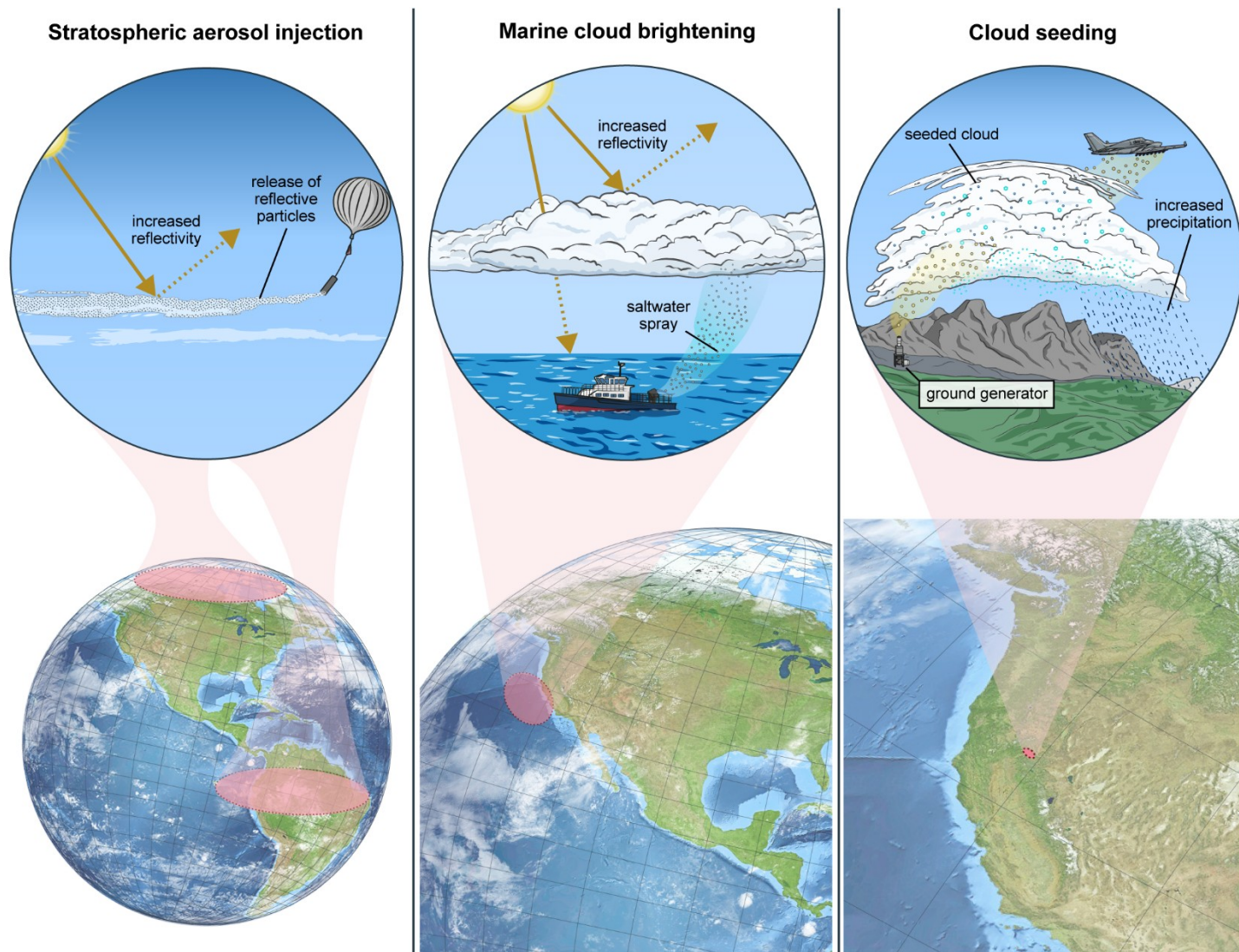
Figure 1: Comparison of Solar Geoengineering for Global or Regional Cooling Versus Cloud Seeding for Increased Local Precipitation
