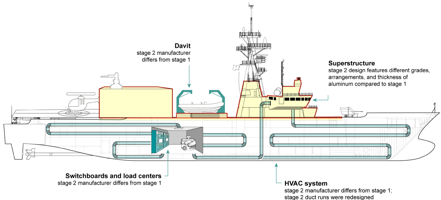
Figure 8: Examples of Differences Between the Offshore Patrol Cutter Designs for Stages 1 and 2
