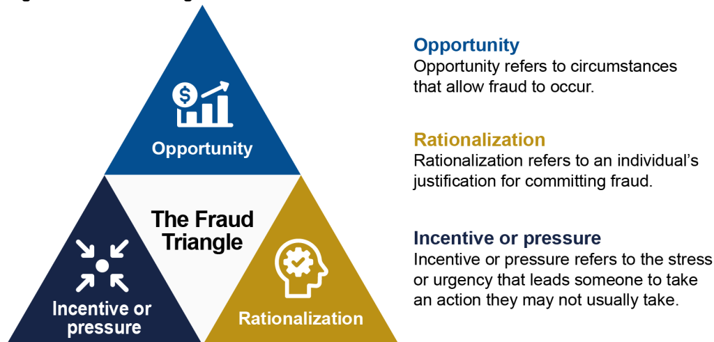
Figure 11: Fraud Triangle
