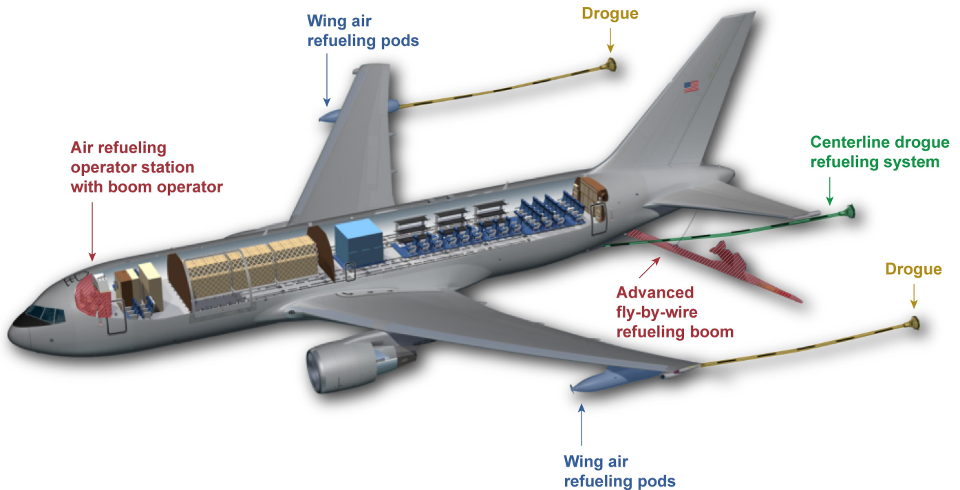
Figure 1: KC-46 Aerial Refueling Subsystems
