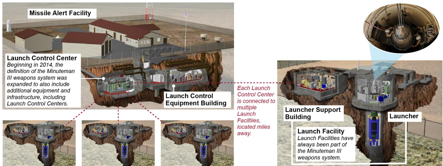
Figure 3: Minuteman III Intercontinental Ballistic Missile Weapon System
