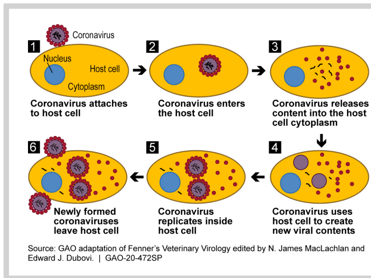
Figure 2. Schematic of how a coronavirus infects host cells. This process is similar for all RNA viruses, the large class to which coronaviruses belong.
