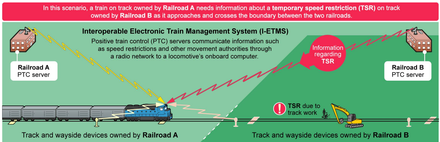
Figure 1: Examples of Positive Train Control (PTC) Interoperability across Different Railroads’ Territories
