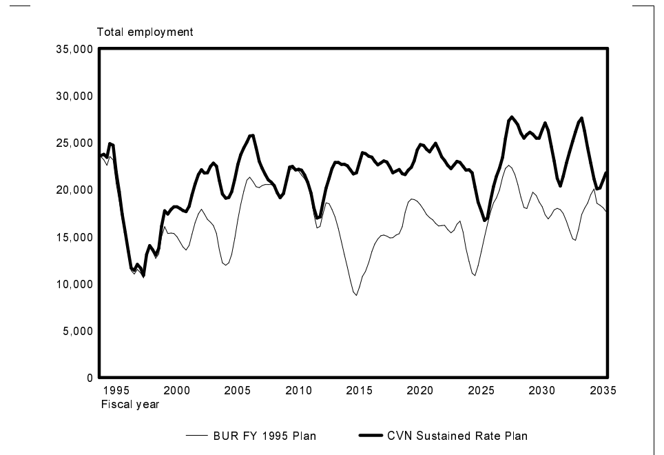
Figure 2.10: Total Employment Level at NNS for Option 2A—Nuclear Carrier Sustaining Rate Strategy
