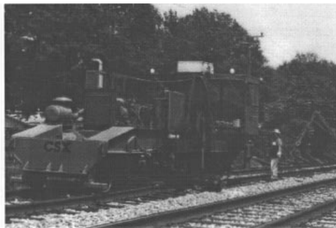
Tie inserter, used to remove and replace wooden ties.
